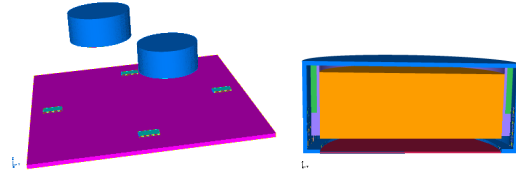
Figure 6. The Gamma detector model (left) and the cross section through one detector (right).
