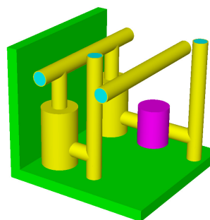
Figure 3. The pipeworks model. The violet body represents the scoring volume. The Neutron source is coloured blue.
